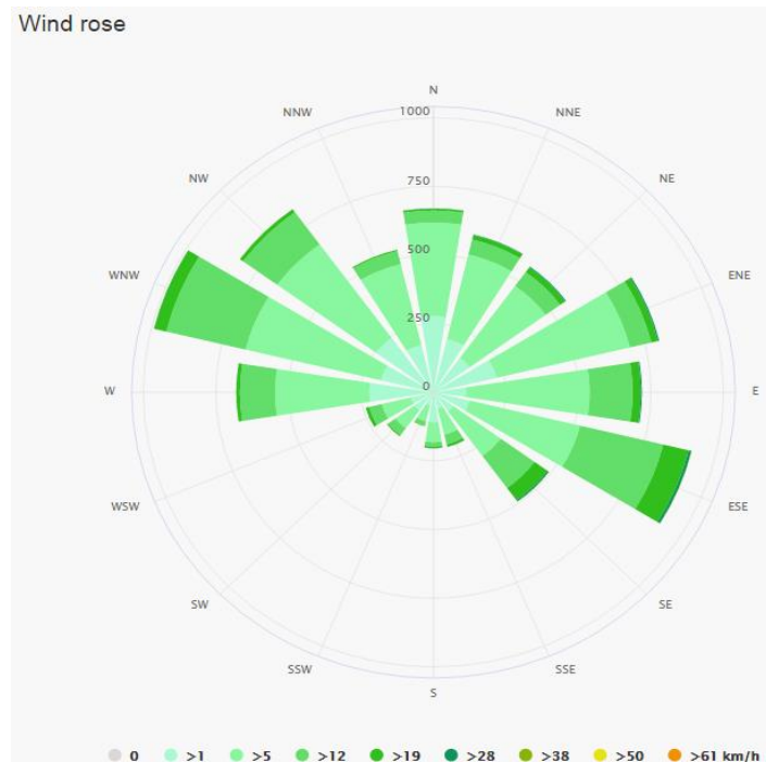
Figure 9: Wind Rose diagram of Sheikhupura
