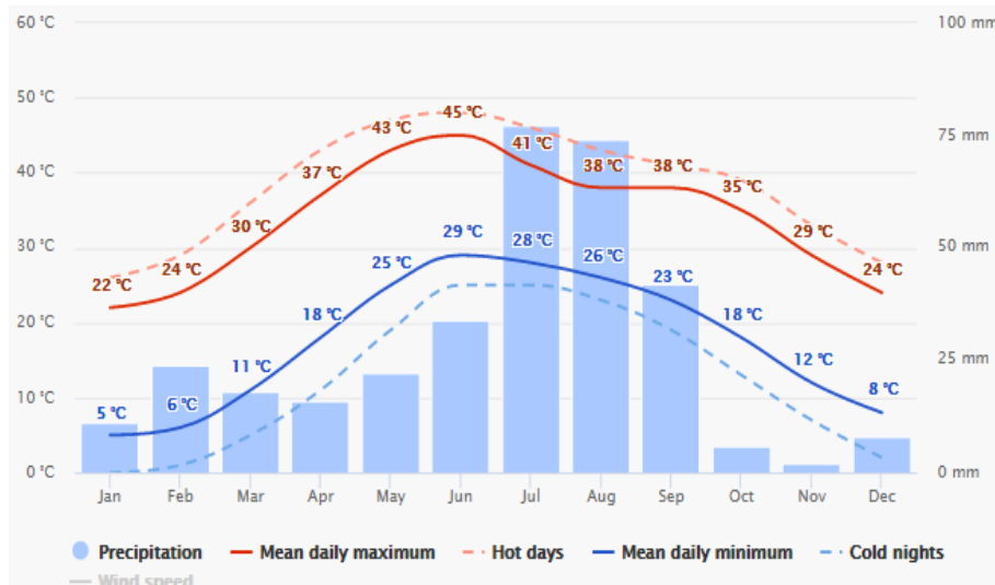
Figure 7: Average Annual Temperatures and precipitation in Sheikhupura
