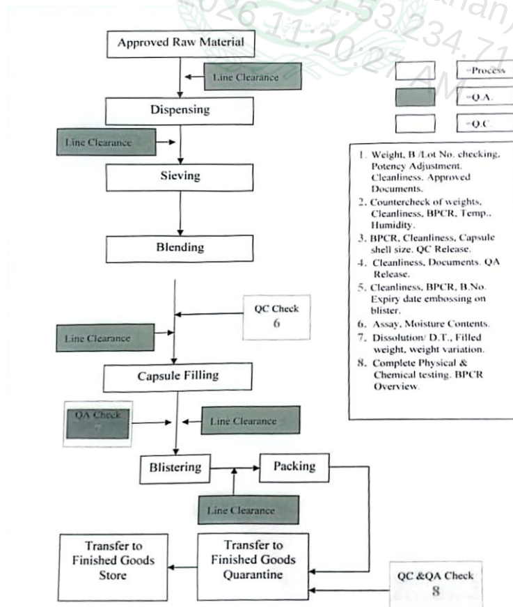
Figure 2: Process Flow for manufacturing of Tablets
