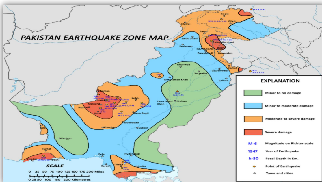
Figure 7: Seismic Zoning of Pakistan
