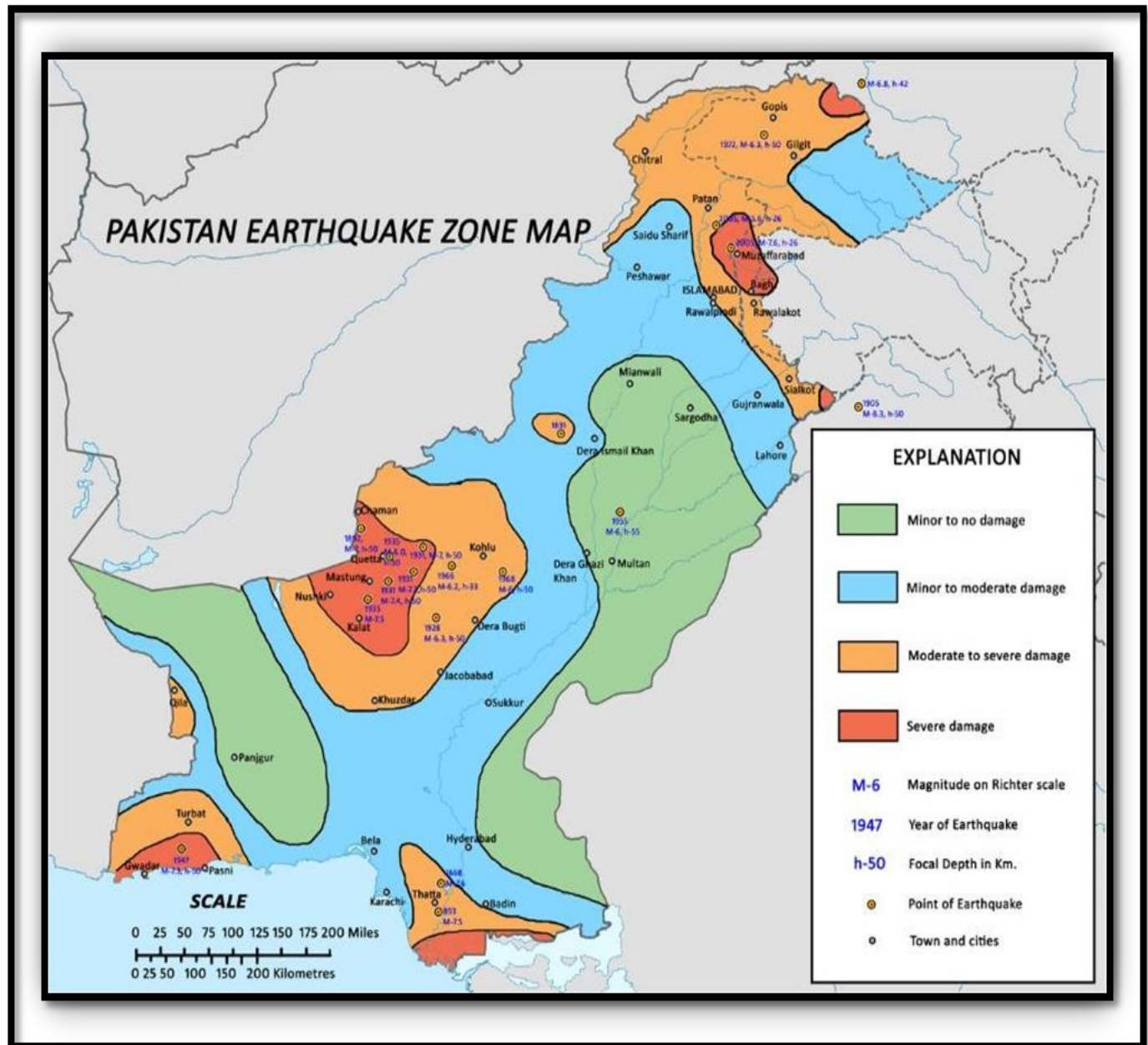
Seismic Zoning of Pakistan
