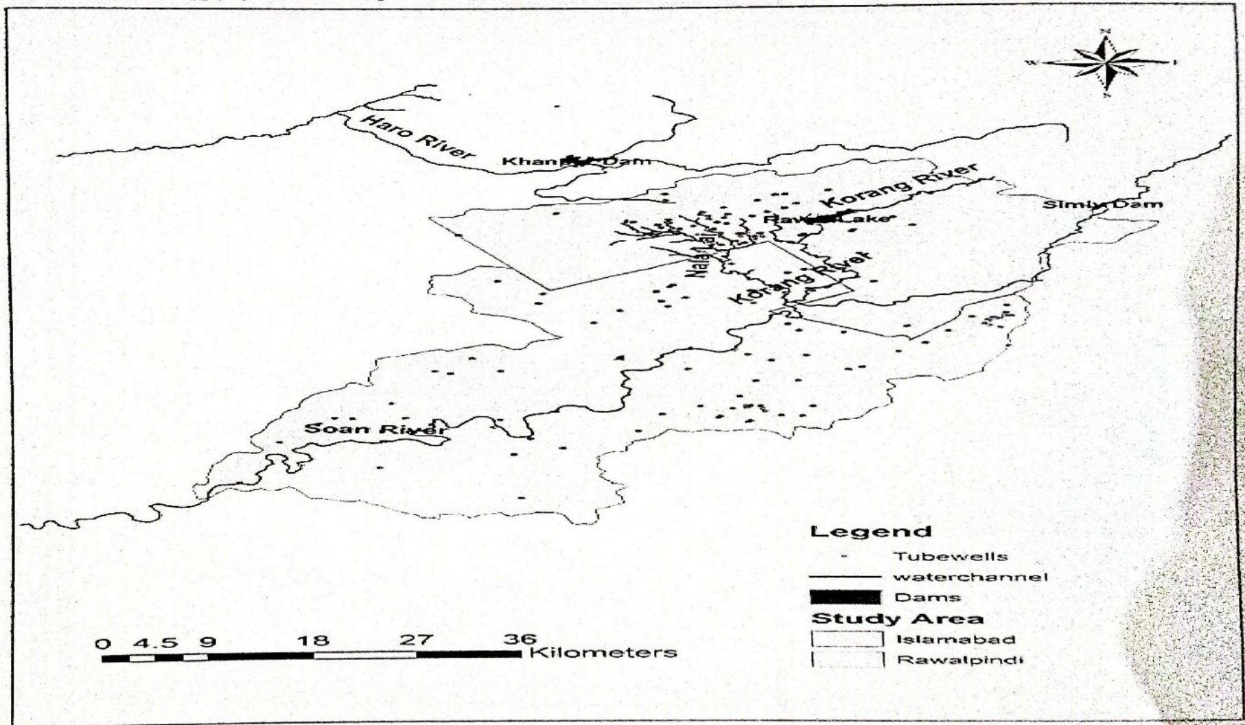
Figure 4.3: Water supply system in Rawalpindi
