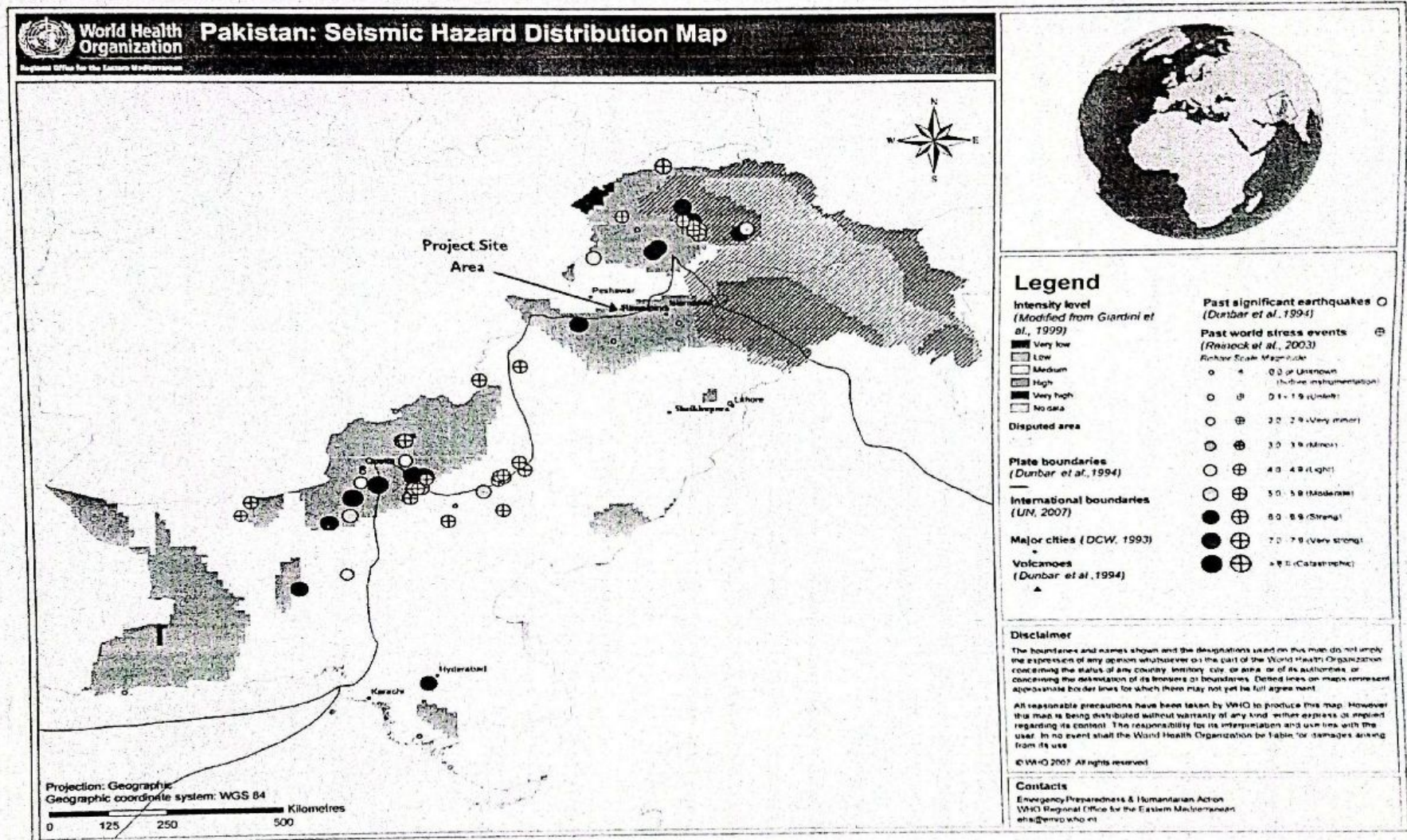
Figure 4.5: WHO Seismic hazard map of Pakistan
