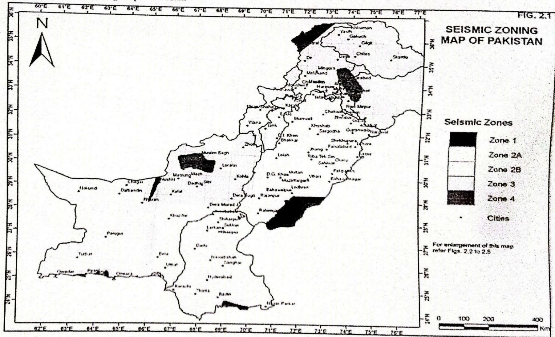
Figure 4.4: Seismic Zoning Map of Pakistan
