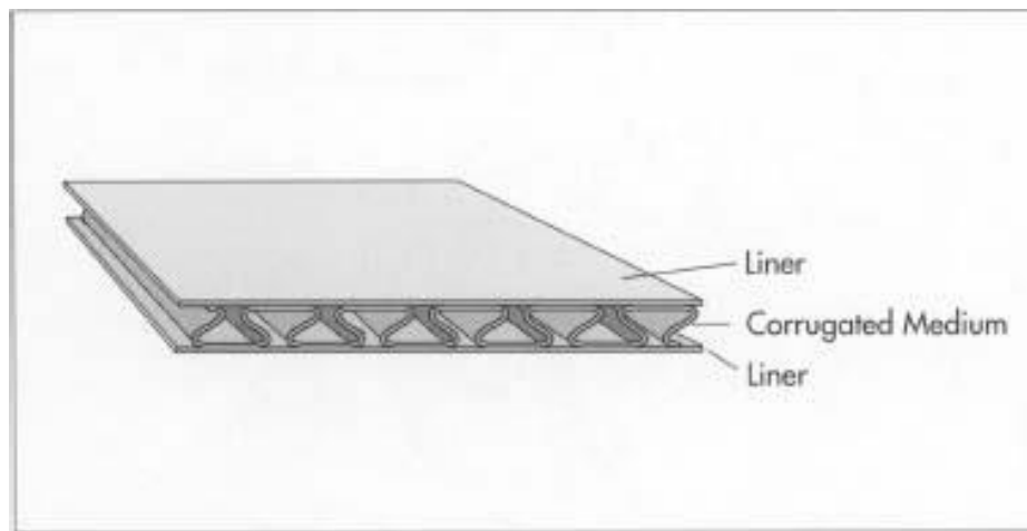
Figure 3-6: corrugated cardboard
