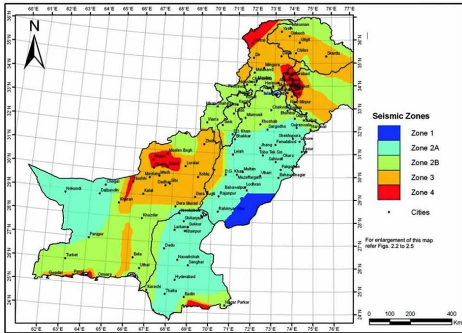
Figure 5-1: Seismic Zoning Map of Pakistan
