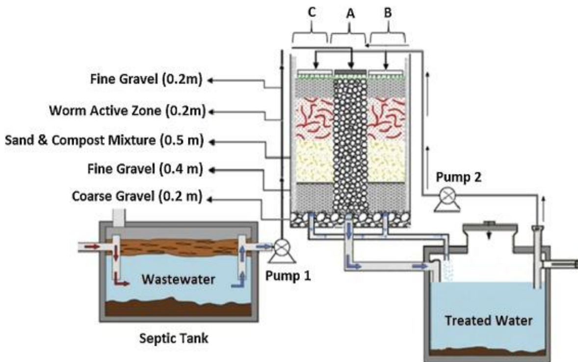
Figure 3-5: Design for Septic Tank
