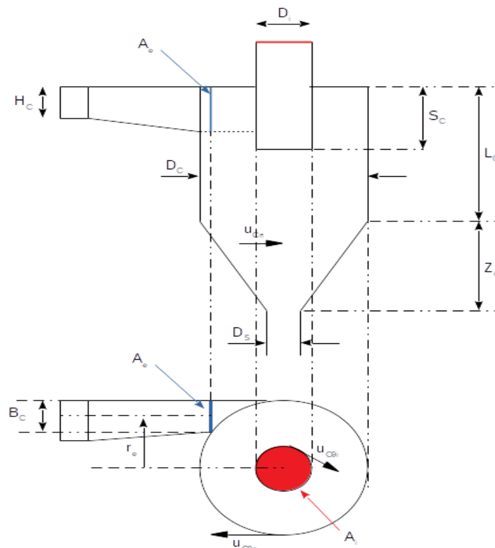
Figure 3-4: Design of Cyclone
