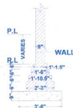
CONSTRUCTIONAL DETAIL OF FOUNDATION WALL
