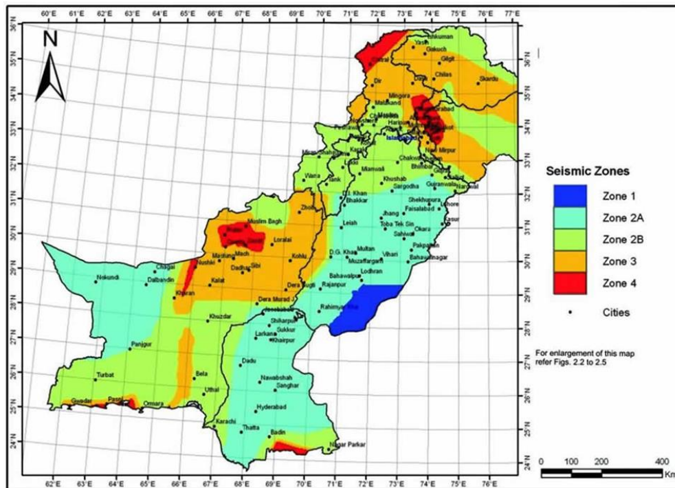
Figure 6: Seismic Zones of Pakistan
