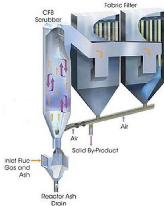
Figure 5: Dry scrubber preliminary design
