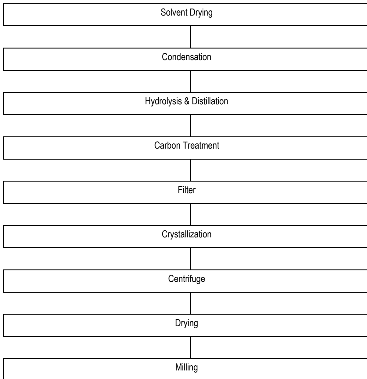
Figure 5: Process Flow for manufacturing of Liquid Base Products
