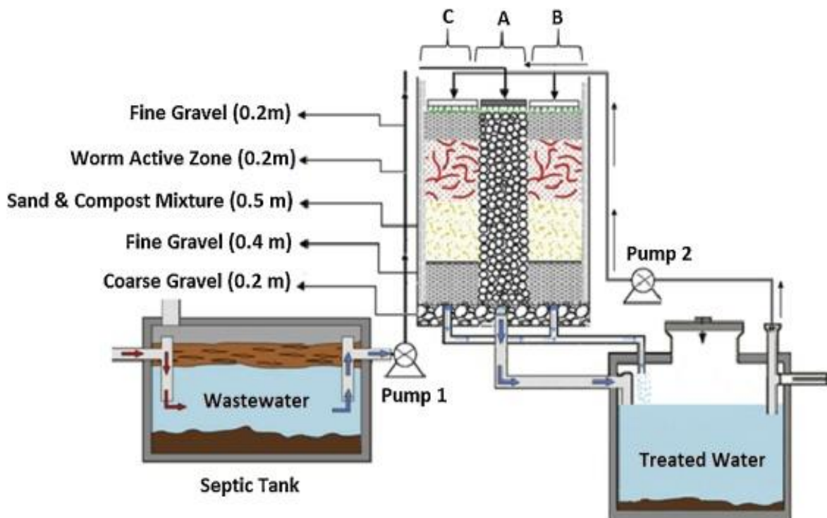
Figure 4: Design for Septic Tank
