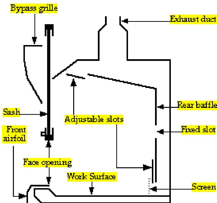
Figure 3: Design of Fume Hood for Air Emission Control Table 5: Specification of Fume Hood
