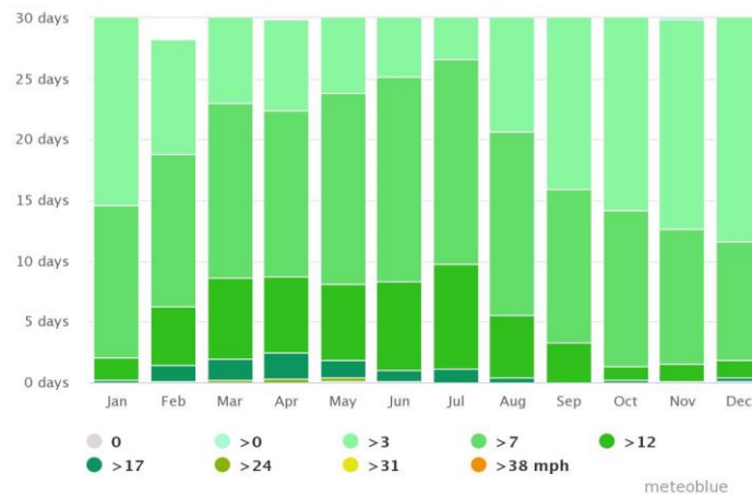
Figure 12: Annual average wind speed in Sheikhupura
