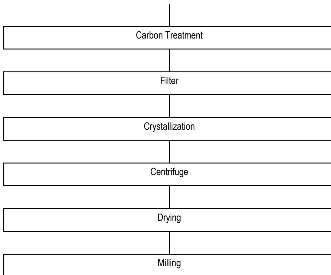
Figure 6: Process Flow for manufacturing of Powder Base Products
