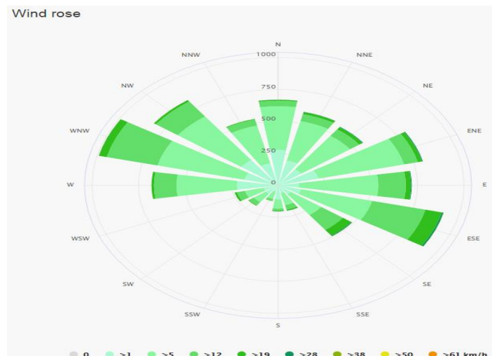
Figure 13: Wind Rose diagram of Sheikhupura
