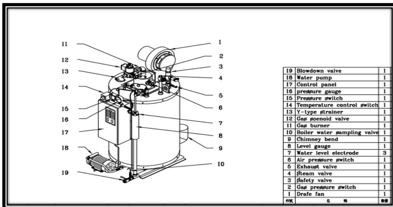
Figure 7: Design of Boiler
