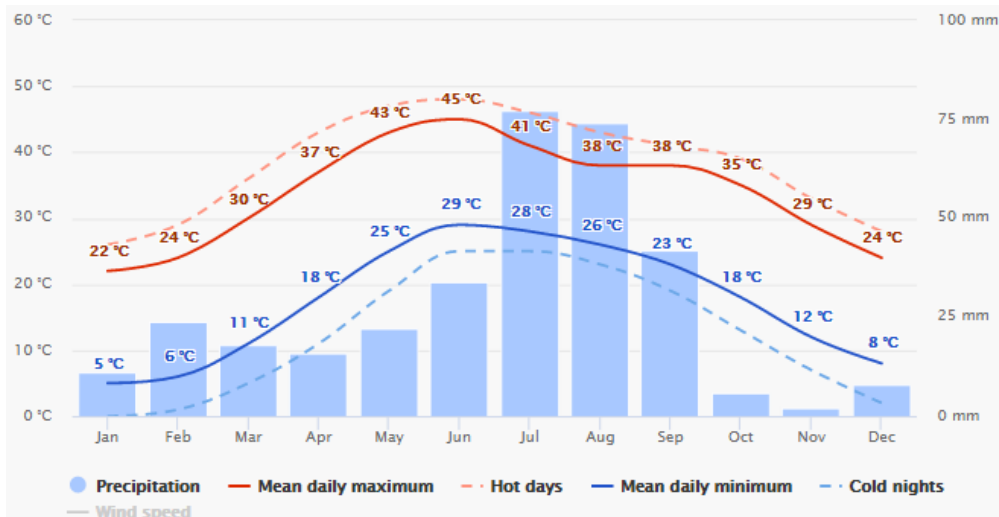
Figure 5: Average Annual Temperatures and precipitation in Sheikhpura
