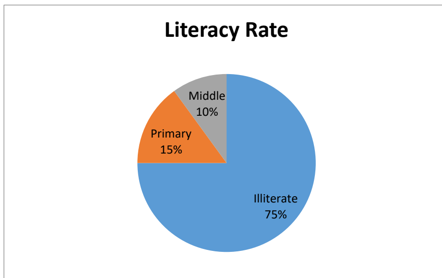
Figure 12: Literacy Rate
