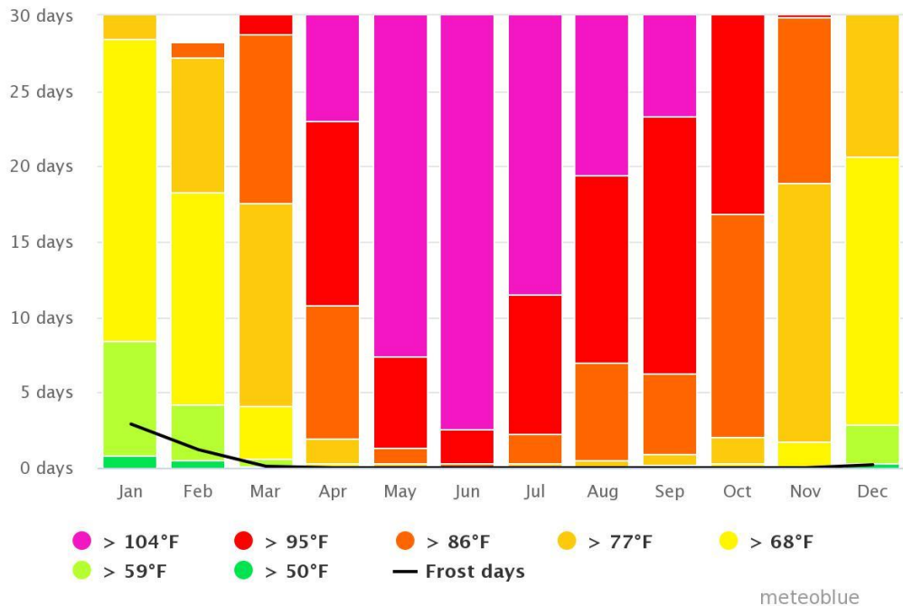
Figure 6: Maximum temperature ranges in Sheikhpura
