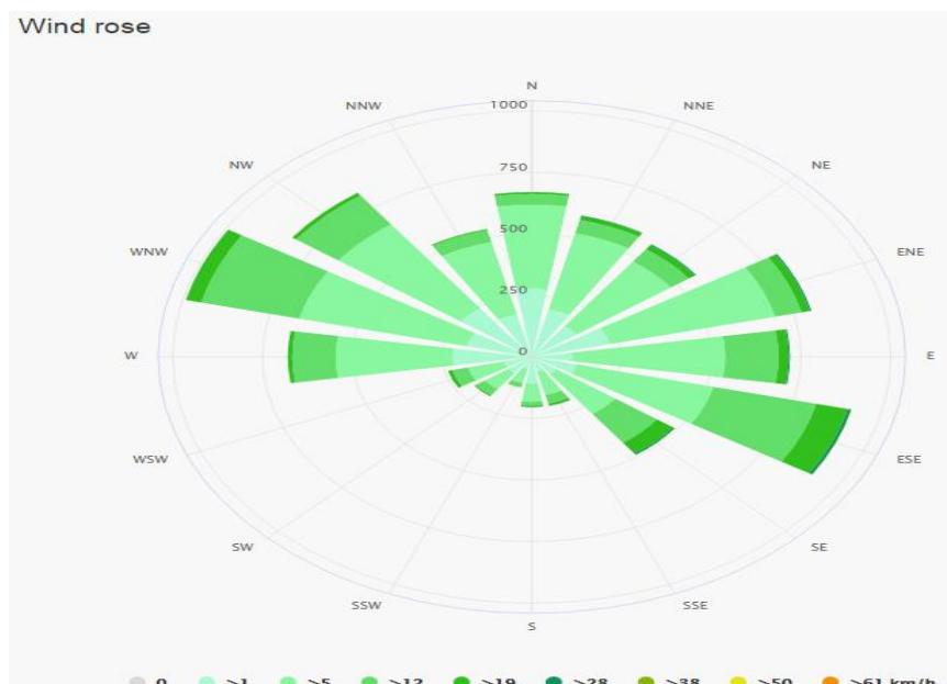
Figure 9: Wind Rose diagram of Sheikhpura
