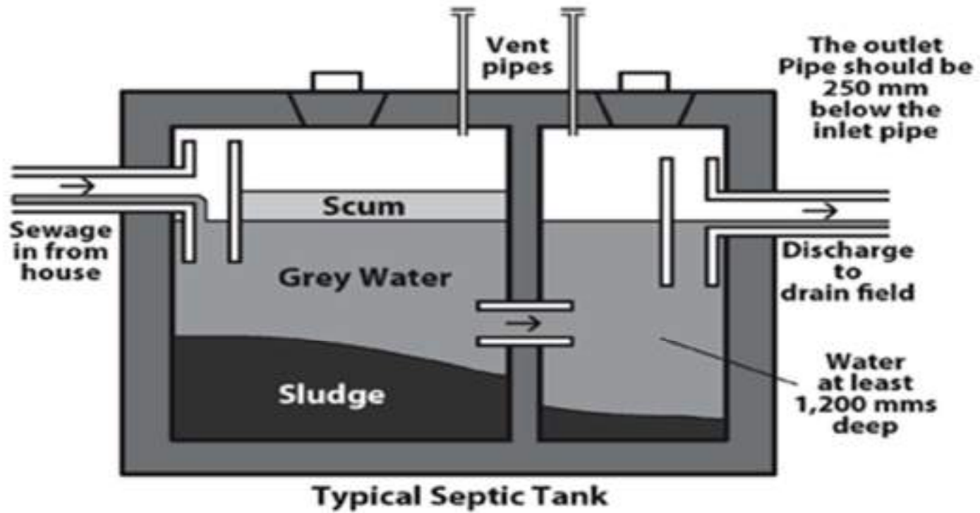
Figure 3.9 Septic Tank
