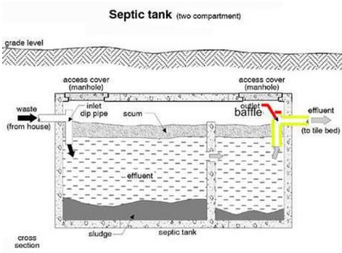
Figure 7-1, Septic Tank
