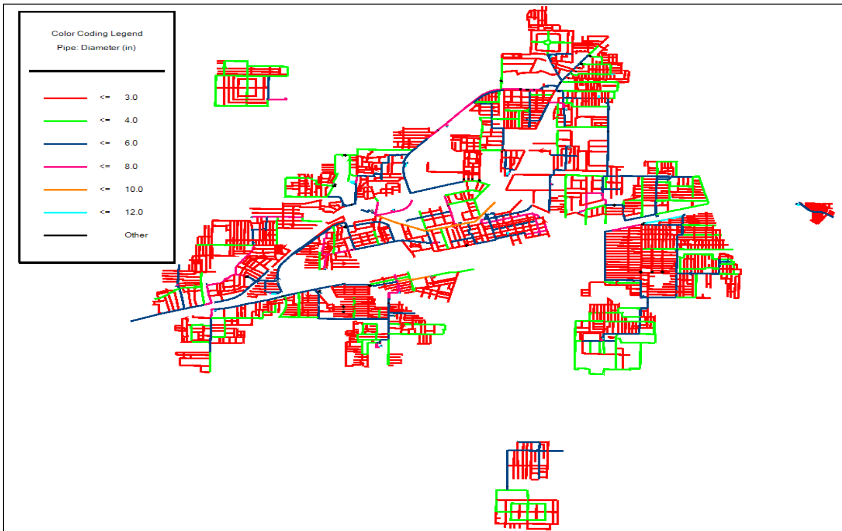
Figure 5-15: Pipe Diameter Of Distribution Network
