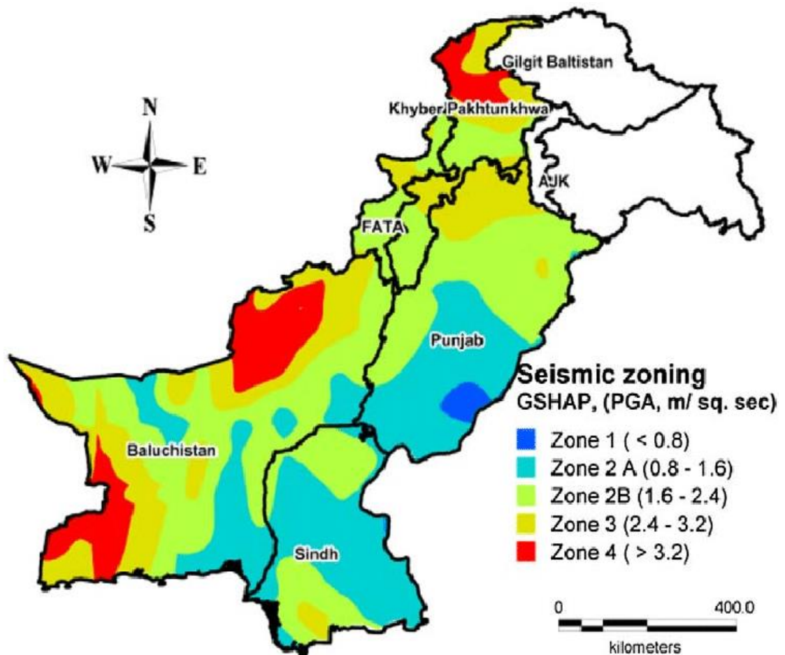
Figure 6-7, Seismic Zones of Pakistan
