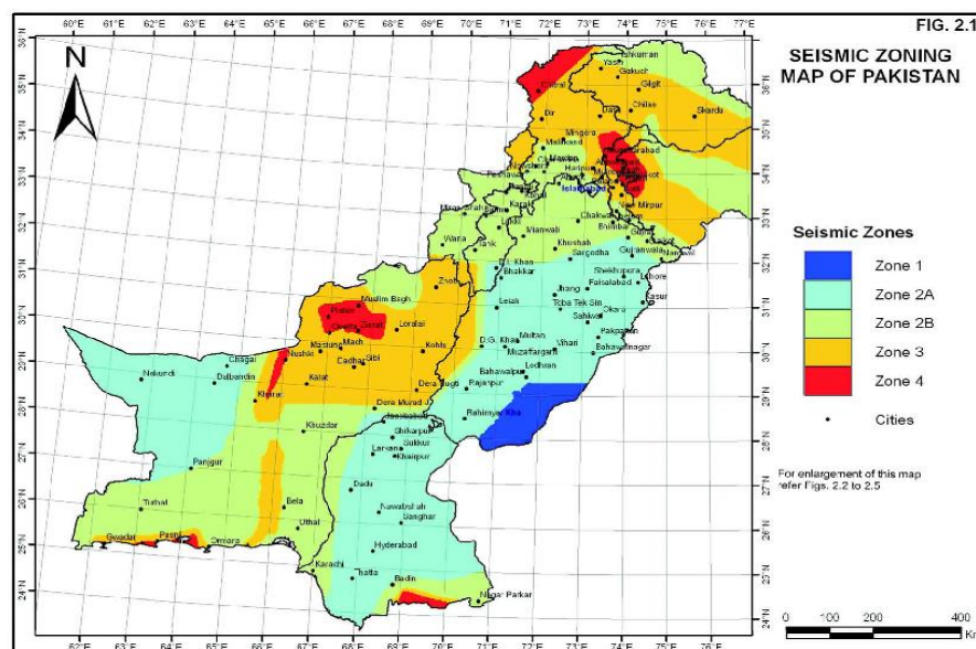
Figure 7: Seismic Zones of Pakistan
