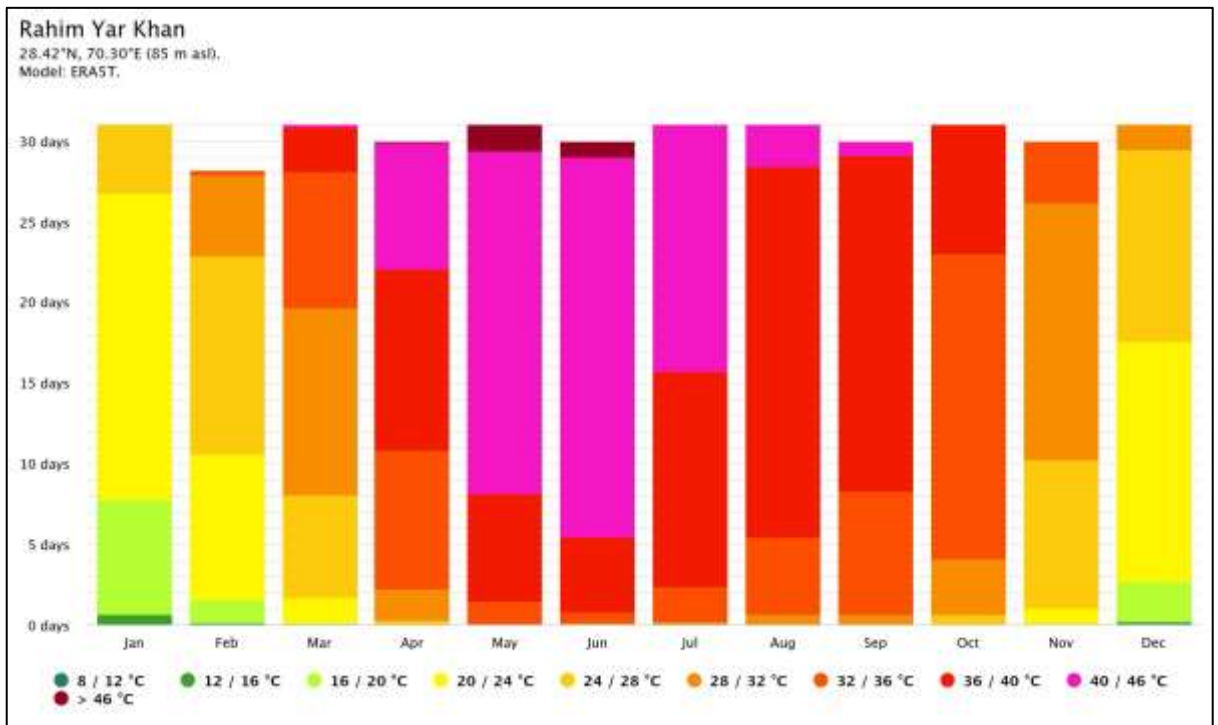
Figure. 6.7: Maximum Temperature
