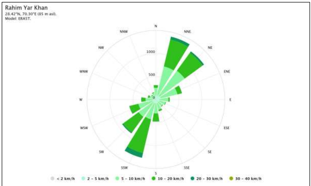
Figure 6.8: Wind Rose
