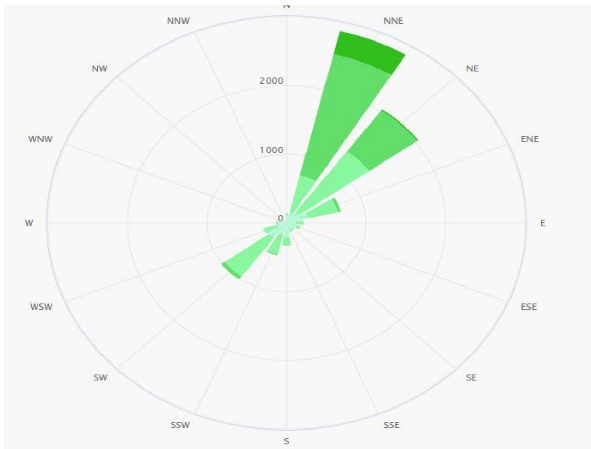
Wind Rose Murree
