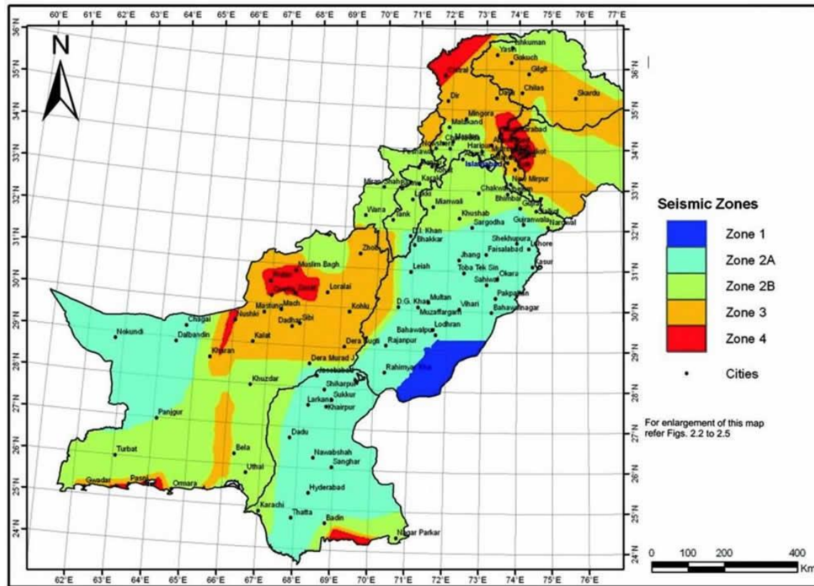
Figure 4-5 Seismic Zoning Map of Pakistan
