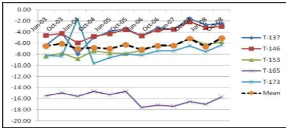
Figure 4-6 Khushab District – Water Table Trends (Feet below GLS)
