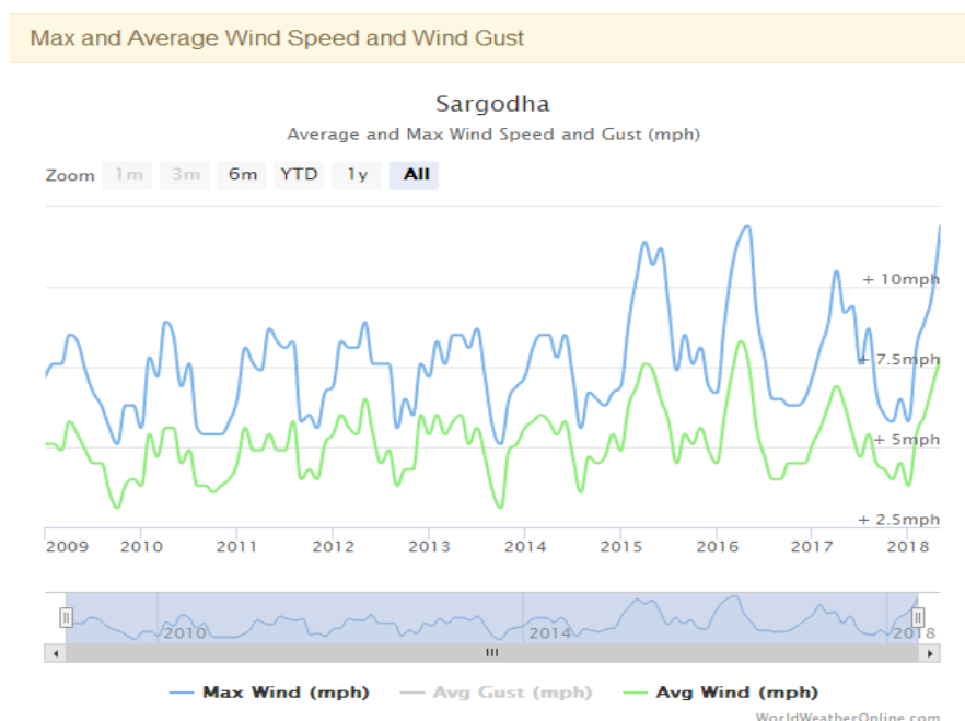
Figure 4-5: Average and maximum Wind Speed of Sargodha Region (Data Source: Worldweatheronline.com, 23-06-2018/3:00 PM)
