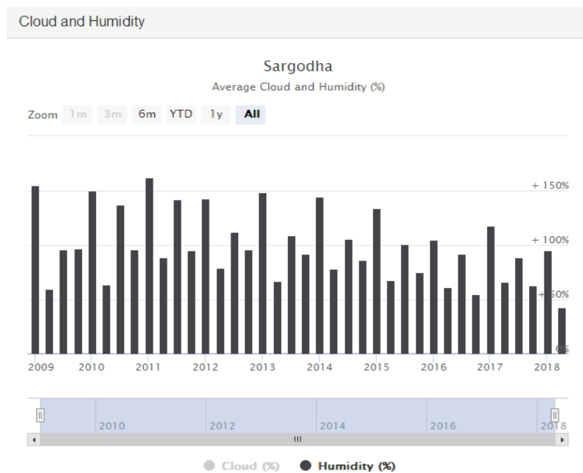
Figure 4-4: Average Relative Humidity of Sargodha Region (Data Source: Worldweatheronline.com, 23-06-2018/3:00 PM)
