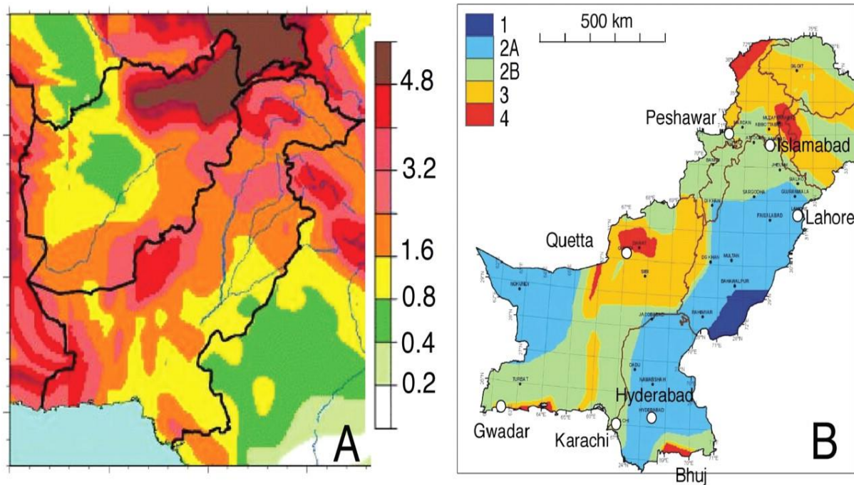
Figure 4-1: Seismic Zone of Pakistan (Geological Survey of Pakistan)
