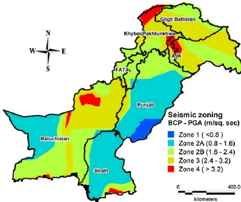
Figure 5-1: Seismic Map of Pakistan
