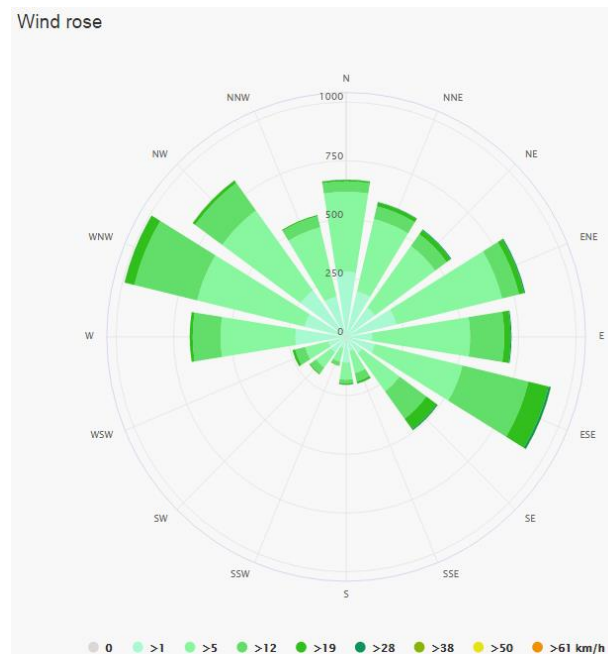
Figure 12: Wind Rose diagram of Sheikhupura
