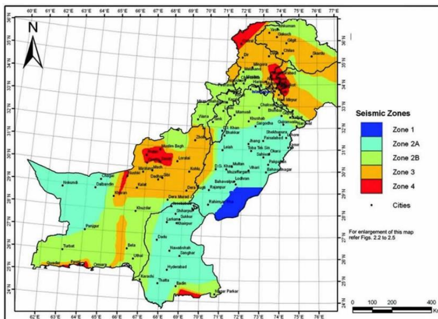
Figure 7: Seismic Zoning Map of Pakistan
