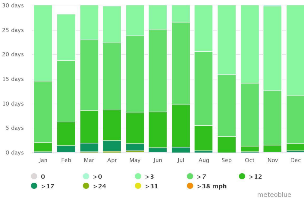
Figure 11: Annual average wind speed in Sheikhupura
