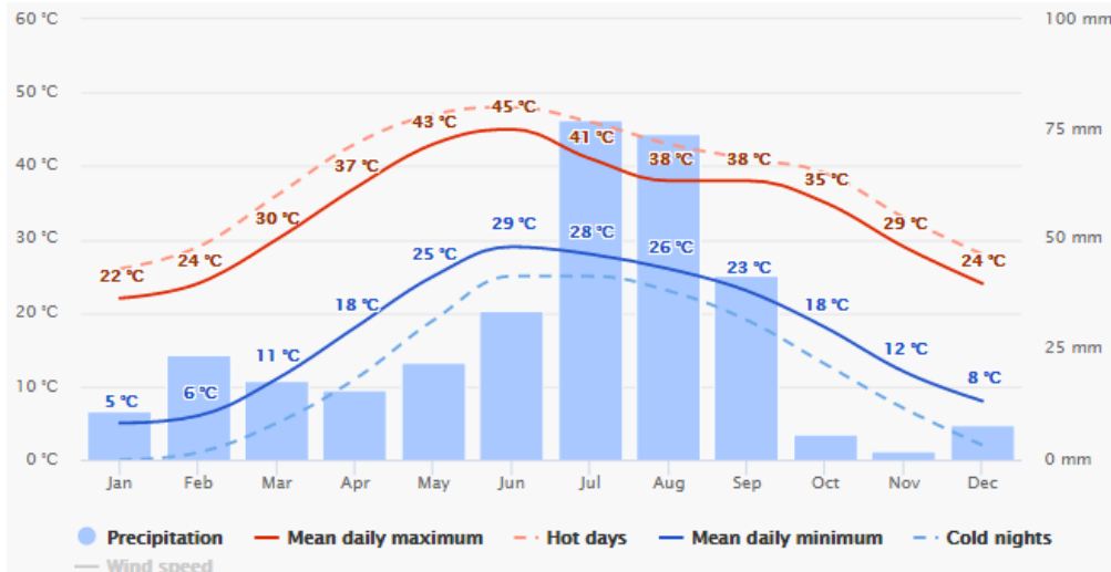
Figure 8: Average Annual Temperatures and precipitation in Sheikhpura
