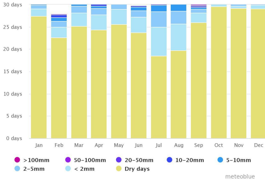
Figure 10: Annual Precipitation amounts in Sheikhupura
