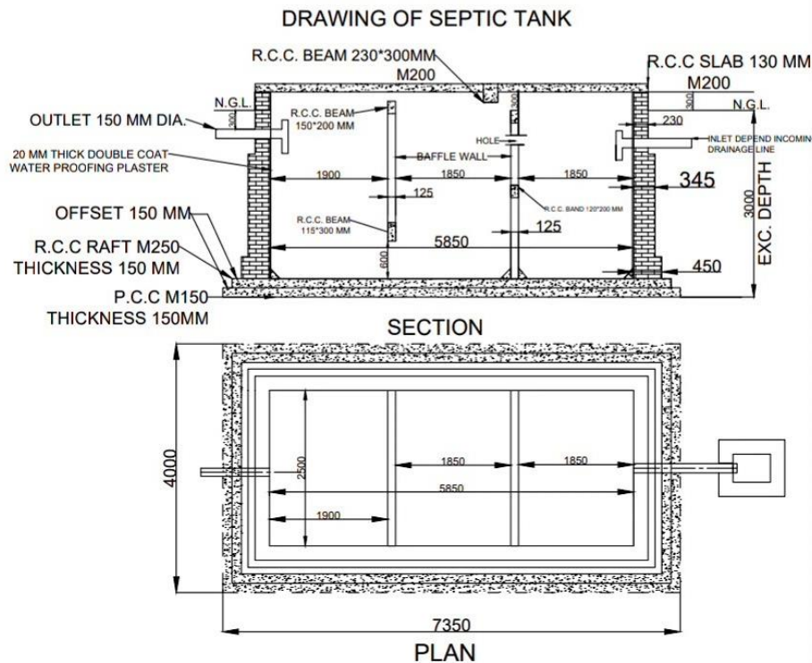
Figure 4: Septic Tank
