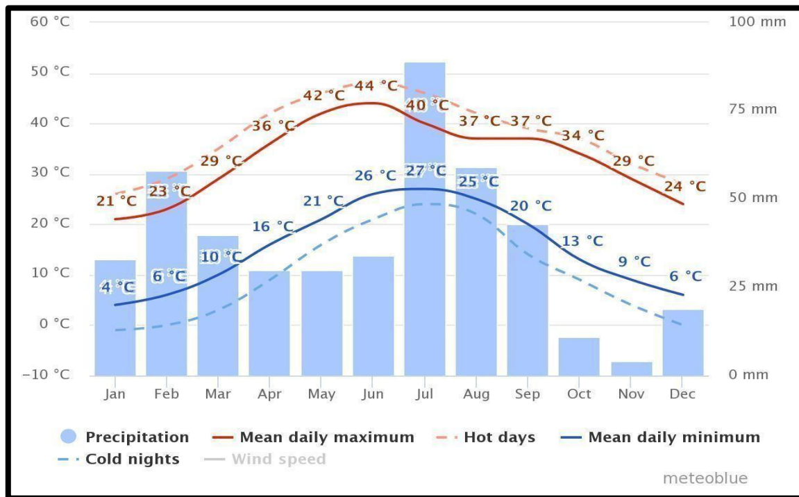
Fig. 4.3: Climatic Conditions of Sheikhupura including Project Area 3
