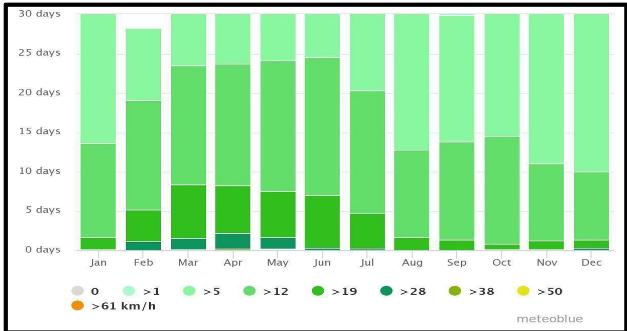
Fig. 4.6: Wind Speed Graph of Sheikhpura 5
