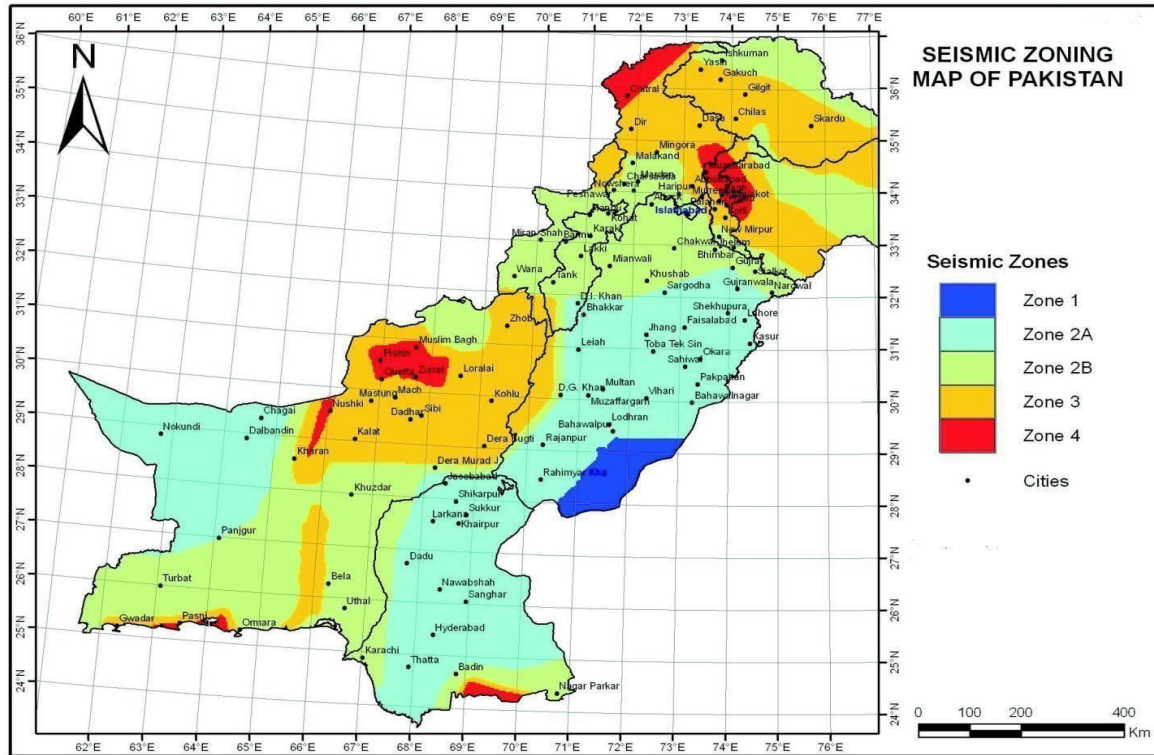
Fig. 4.7: Seismicity Map of Pakistan
