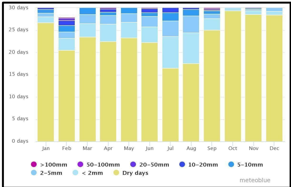
Fig. 4.4: Climatic Conditions (Monthly Precipitation Chart) 4
