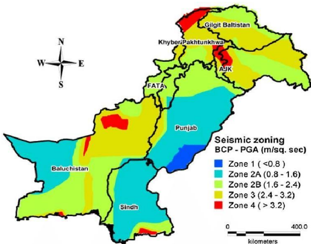
Figure 4 Seismic Zone of Pakistan
