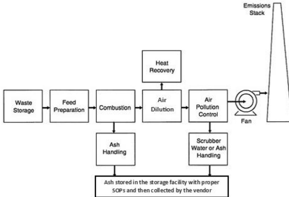
Figure 4 General process diagram
