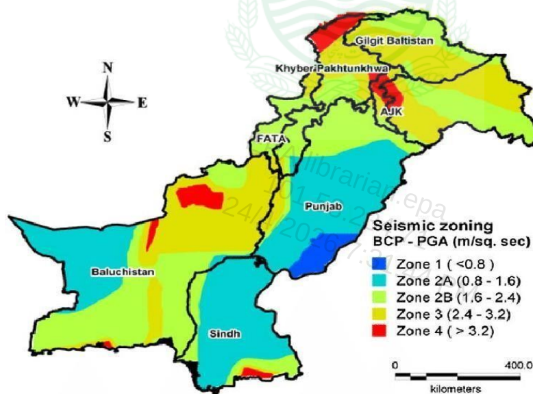
Figure 3-1: Seismic Zoning of Pakistan
