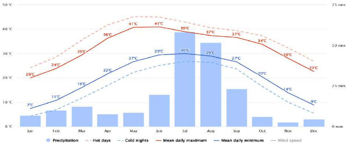
Figure 6-3, Average Annual Maximum and Minimum Temperature, and Precipitation – Bahawalpur
