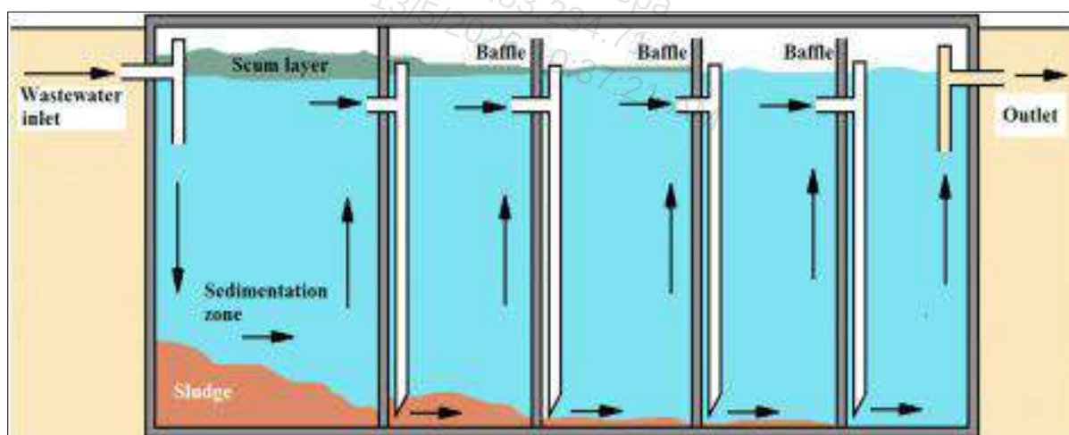
Figure 5-9, Layout Plan of ABR
