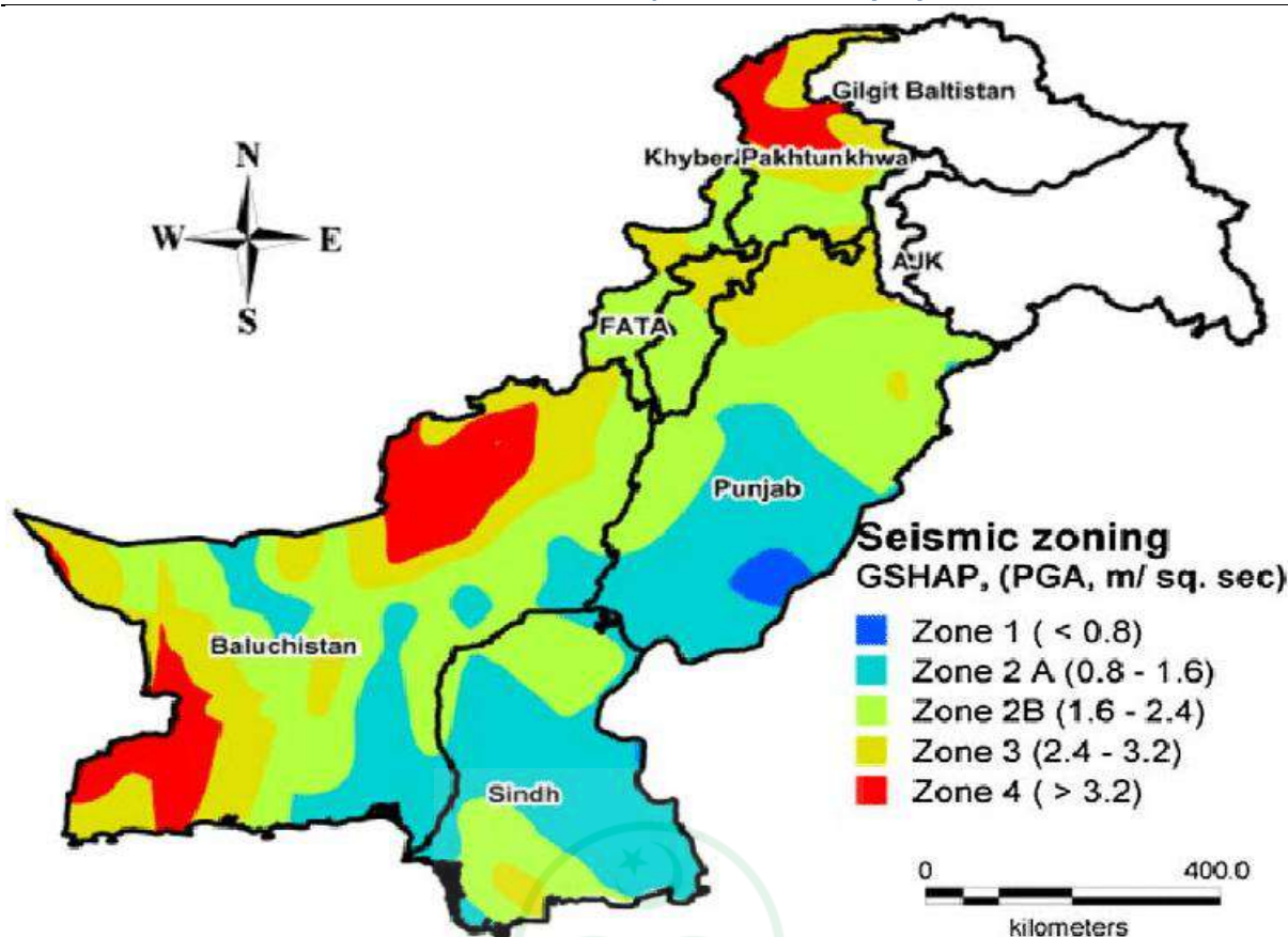
Figure 6-7, Seismic Zones of Pakistan
