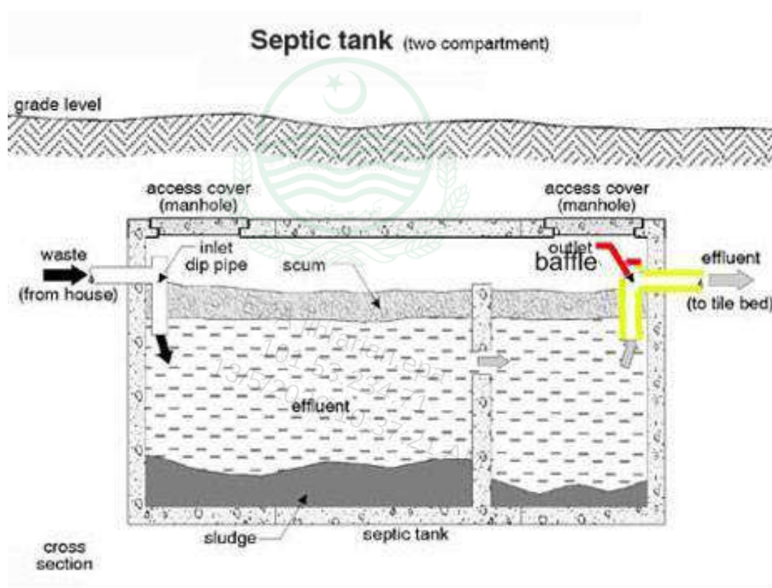
Figure 7-1, Septic Tank
