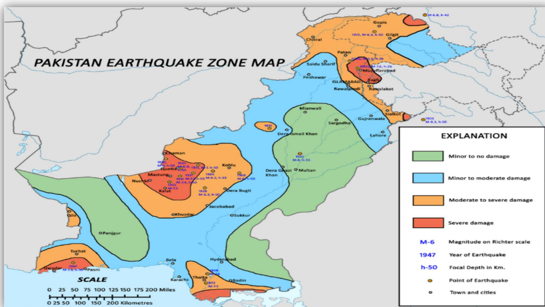
Figure 6: Seismic Zoning of Pakistan
