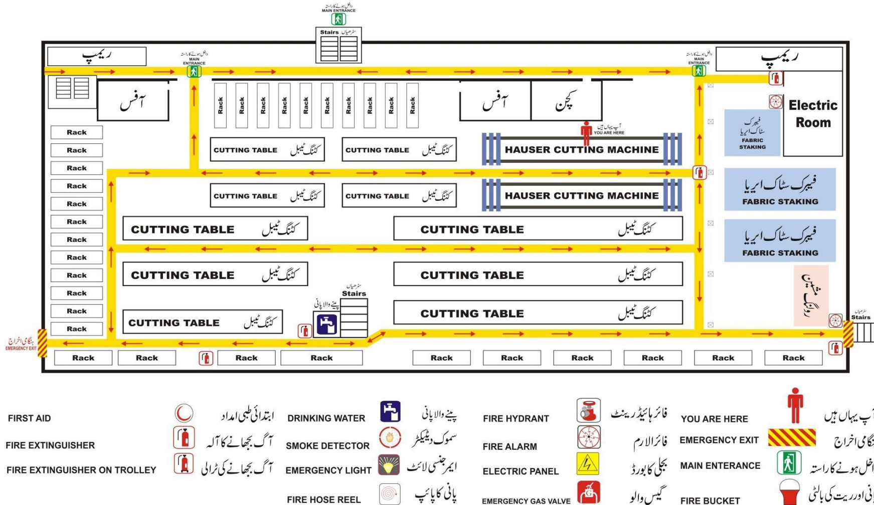
Figure 16: Emergency Evacuation plan of Hauser Cutting
