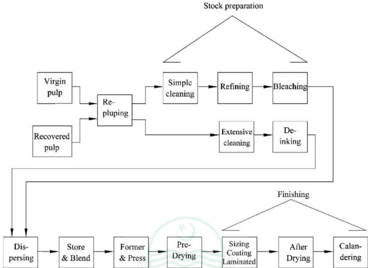
Figure 6: Paper manufacturing process flow diagram
