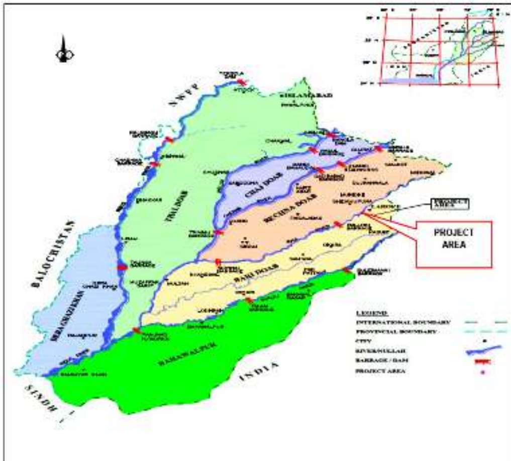
Figure 3.5: Hydrology of the project area
