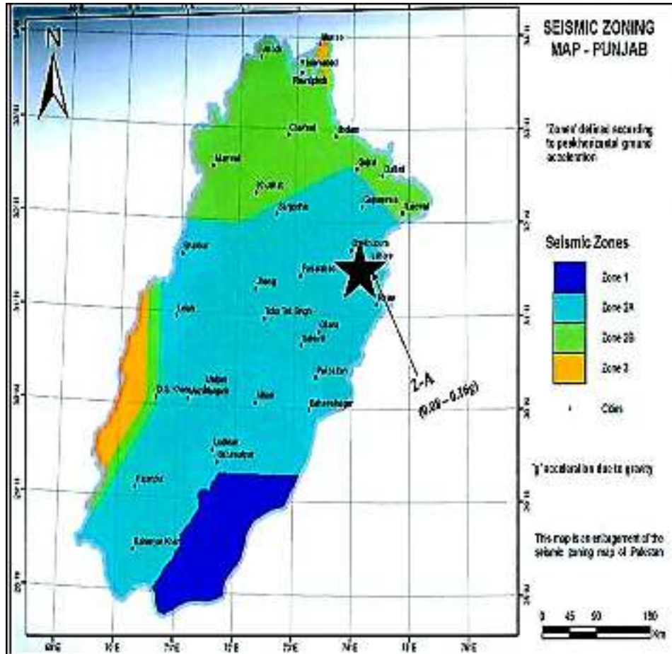
Figure 3.4: Seismic Zoning of Punjab
