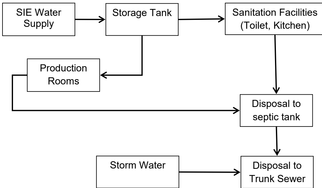
Figure 4.1: Water Flow Diagram
