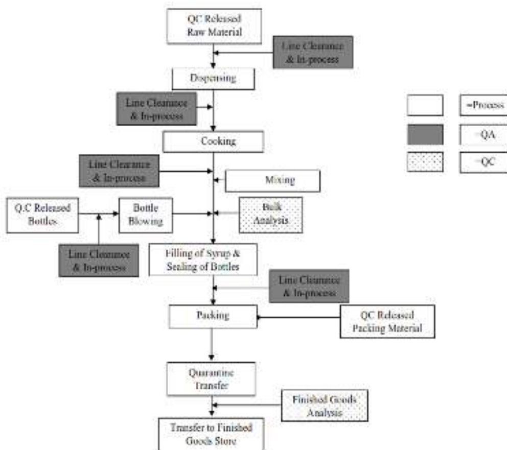
Figure 2.5: Syrup Manufacturing Process Flow
