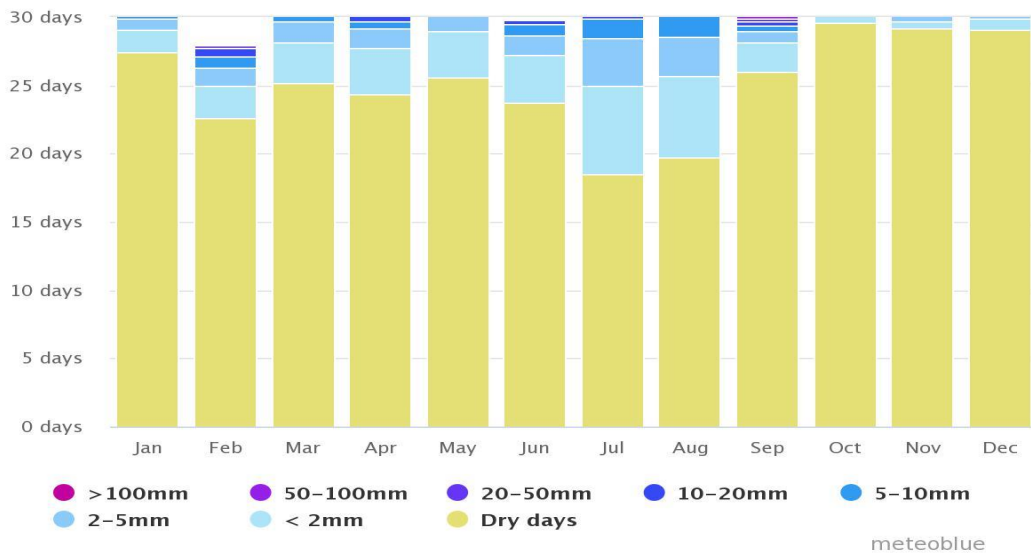
Figure 9: Annual Precipitation amounts in Sheikhupura
