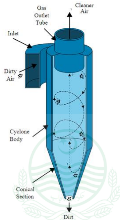
Figure 3: Cyclone for Air Emission Control
