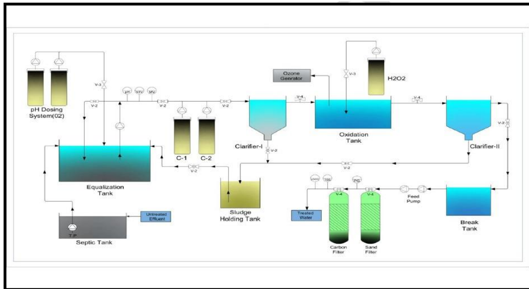
Figure 4: Design of Cyclone
