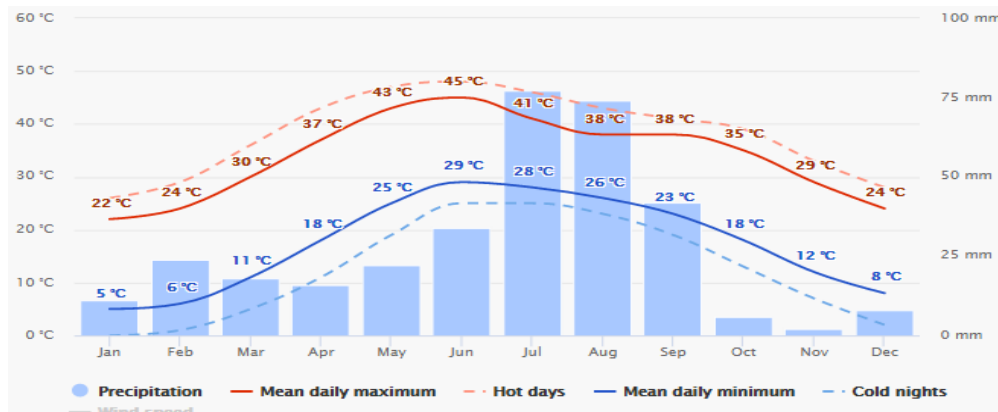
Figure 7: Average Annual Temperatures and precipitation in Sheikhpura
