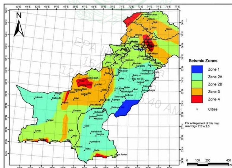
Figure 6: Seismic Zoning Map of Pakistan
