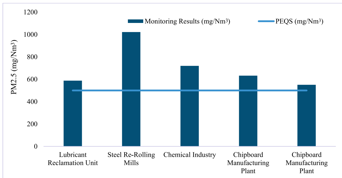
Figure 2-12 Monitoring of industrial emissions of PM (mg/Nm 3 )
