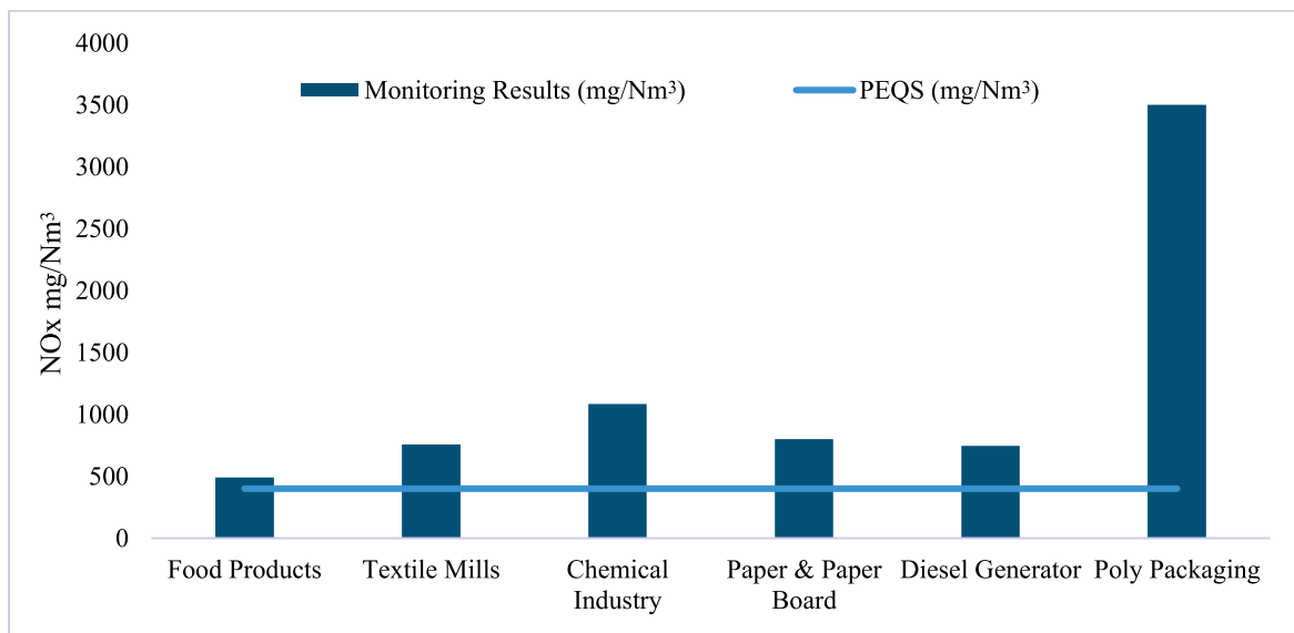
Figure 2-11: Monitoring of industrial emissions of NO x (mg/Nm 3 )
