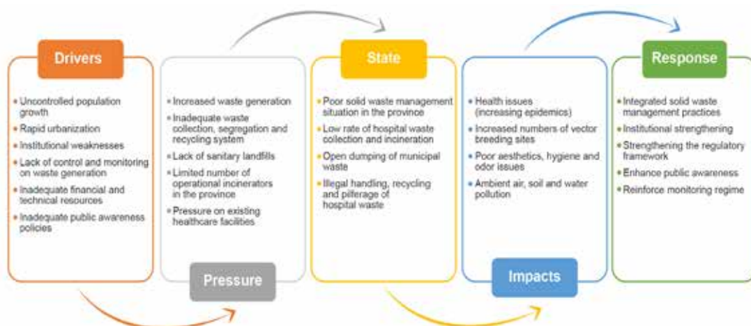
Figure 5-16 DPSIR framework
