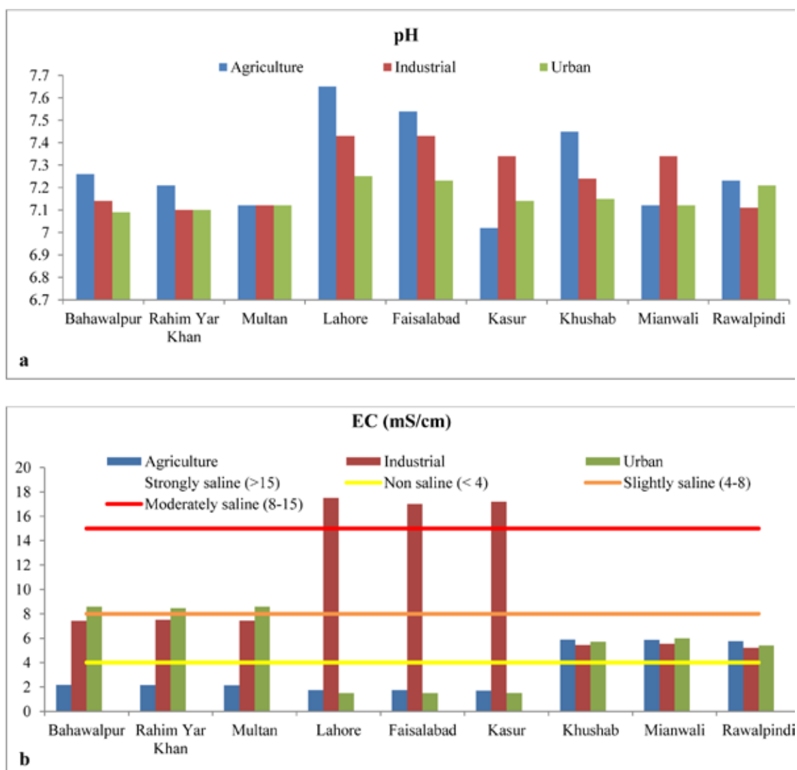
Figure 4-4 pH (a) and EC (b) in three soil types of selected districts in Punjab
