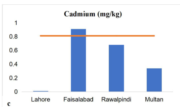
Figure 5-8: Results of Soil Analyses in study area (values compared with USEPA Standards for soil quality)
