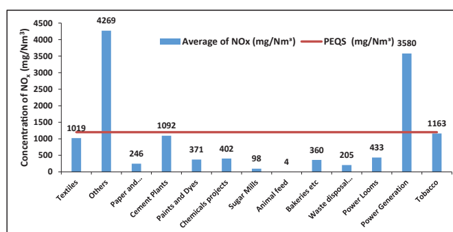
Figure 3-12: Average \text{NO}_x in stack emissions of various industries
