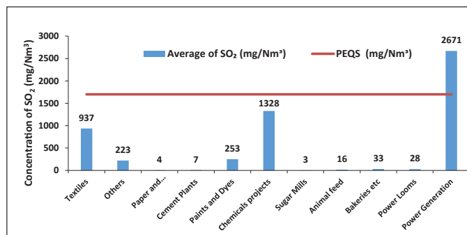
Figure 3-13: Average \text{SO}_2 in stack emissions of various industries
