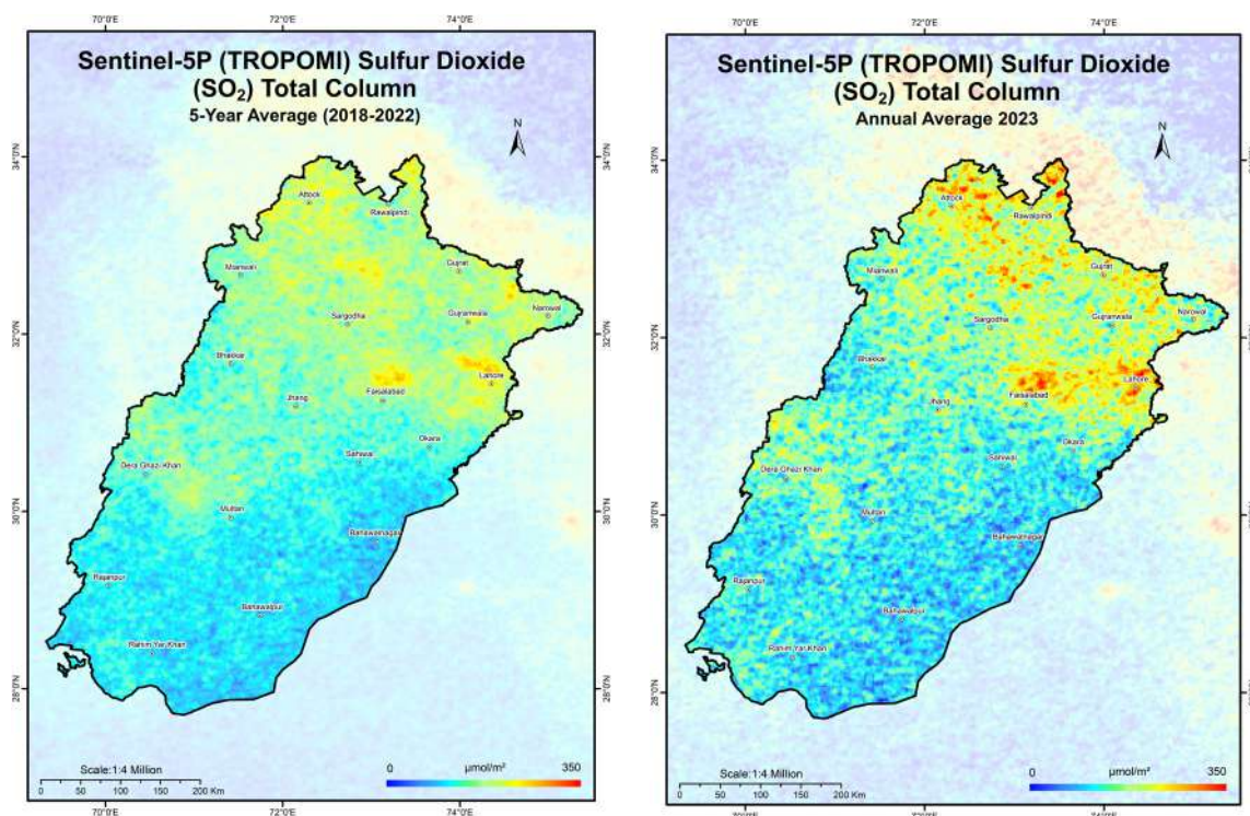
Figure 3-11: Comparison b/w baseline (5-Year averaged) and annual averaged concentration of SO 2 (μmol/m 2 )
