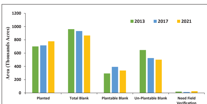
Figure 2-6: Forest Cover Change in Punjab
