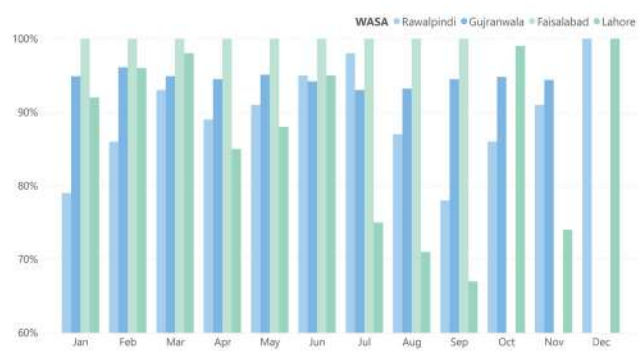
Figure 4-11: Biological fitness of drinking water in distribution systems
