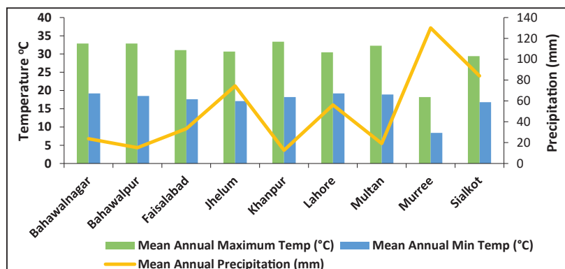
Figure 6-1: Climate Normals in Punjab (1991-2020)
