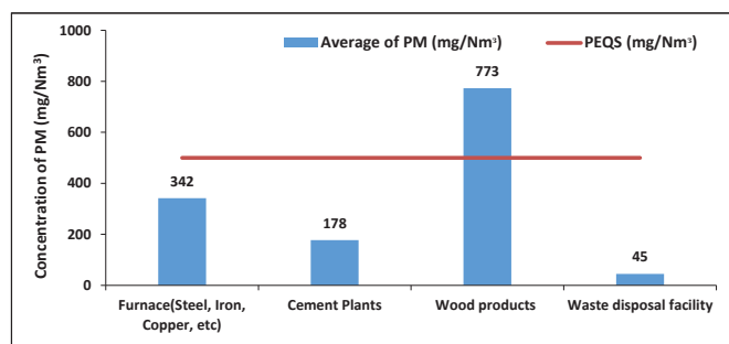
Figure 3-14: Average \text{PM} concentration in stack emissions of various industries
