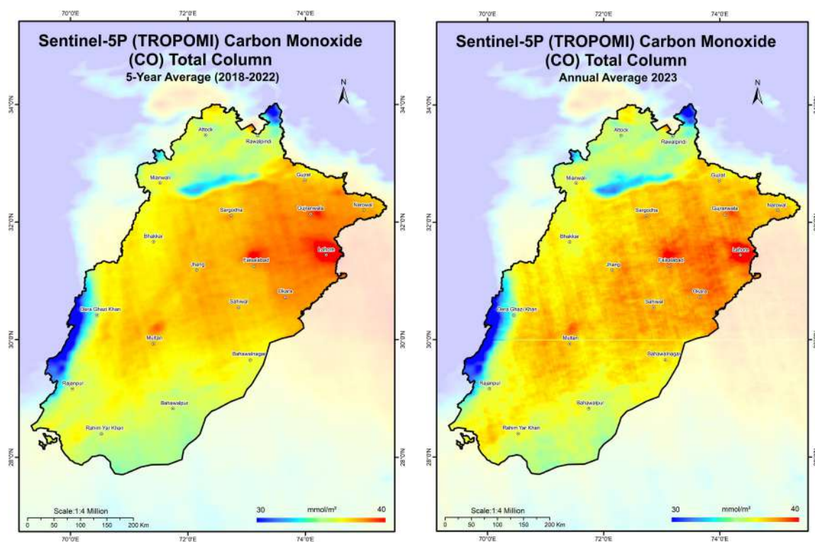
Figure 3-9: Comparison b/w 5-Year baseline (2018-2022) and annual averaged (2023) total column concentration of CO ( \text{mmol/m}^2 )
