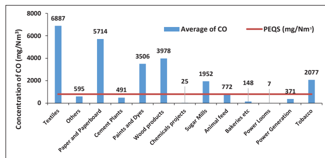
Figure 3-15: Average \text{CO} concentration in stack emissions of various industries
