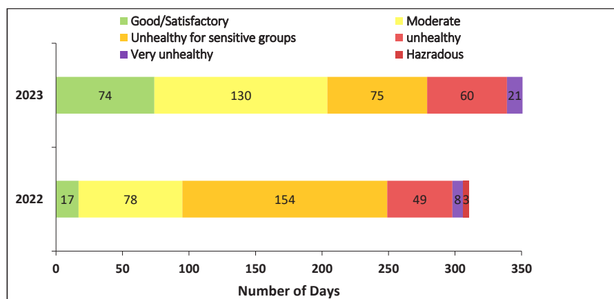
Figure 3-6: Number of days with respect to AQI (PM 2.5 ) air quality in Lahore in 2022 and 2023
