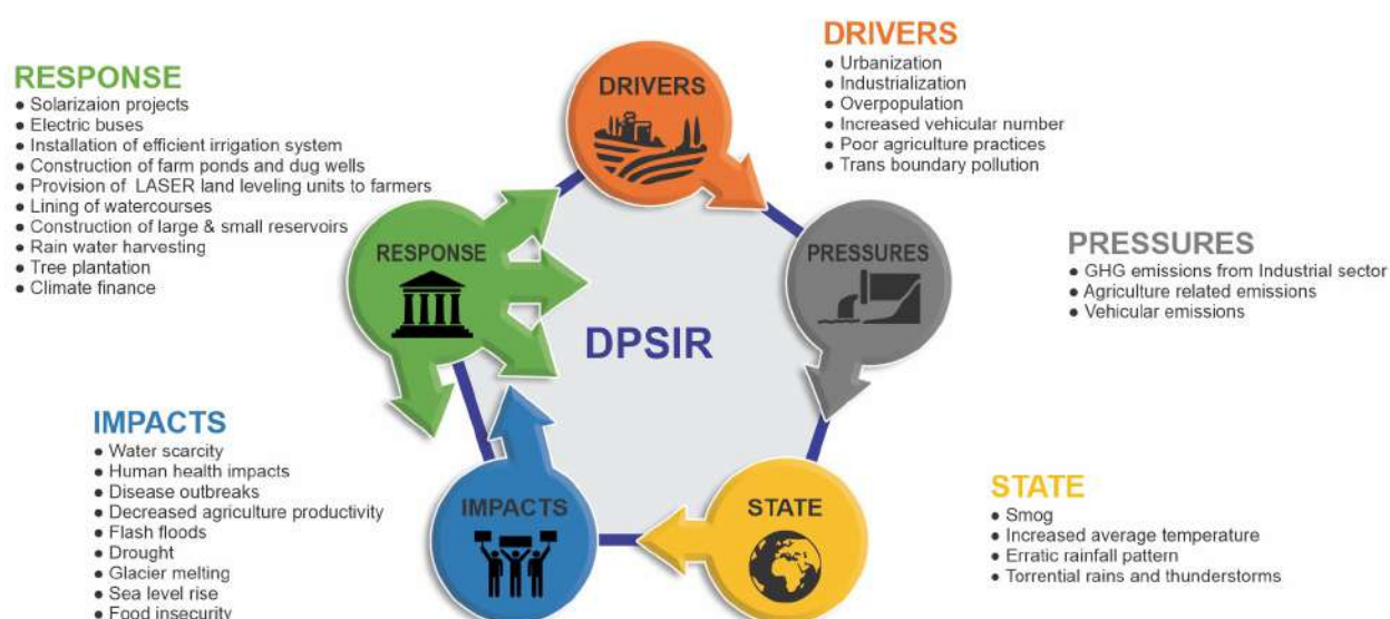
Figure 6-14: DPSIR framework for climate change in Punjab
