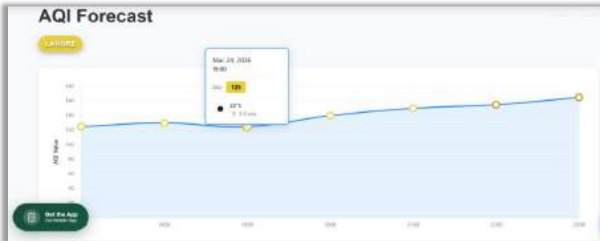
Figure 13.18: Forecasted AQI for next 24 hours — EPA Punjab
