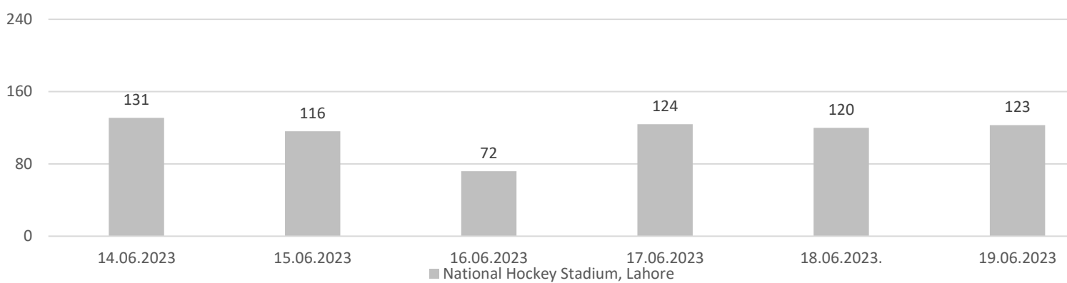
AQI Recorded With AQMS
